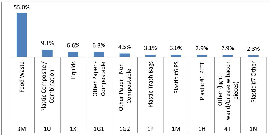
Figure 5-19 ATL – Terminal A19
